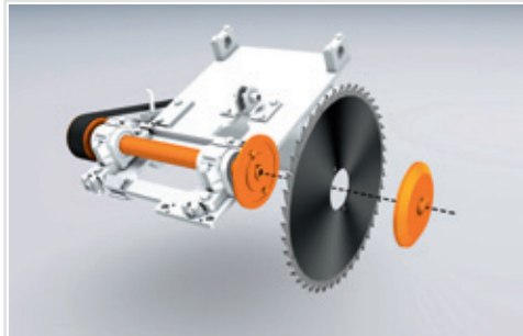
EasyFix – saw blade fast-release system
