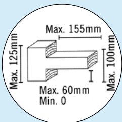
Straight Shoulder Tenon
