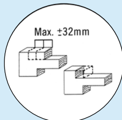
Staggered Tenon
