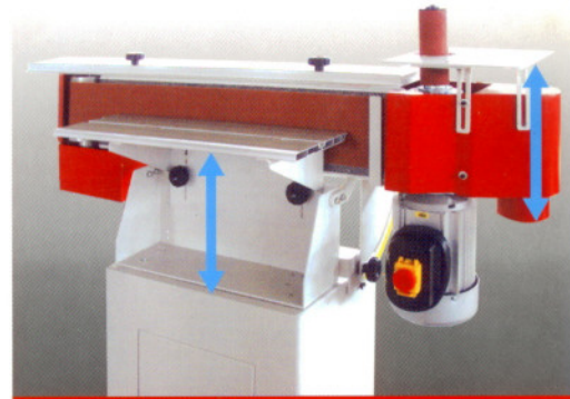
Both tables can be moved up and down.
